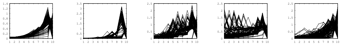
(a) IGD + -EMOA (b) MOMBI-II (c) NSGA-III (d) RVEA (e) MOEA/DD Figure 8.7: Graphical representation of the final set of solutions obtained by the five MOEAs used in our study on DTLZ5 with 10 objectives.
