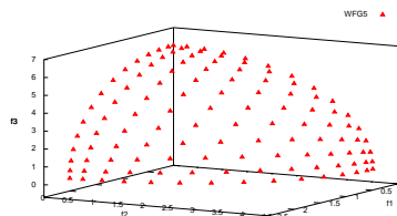
Figure 5.4: Solutions obtained by IGD^+ -EMOA for WFG5.
