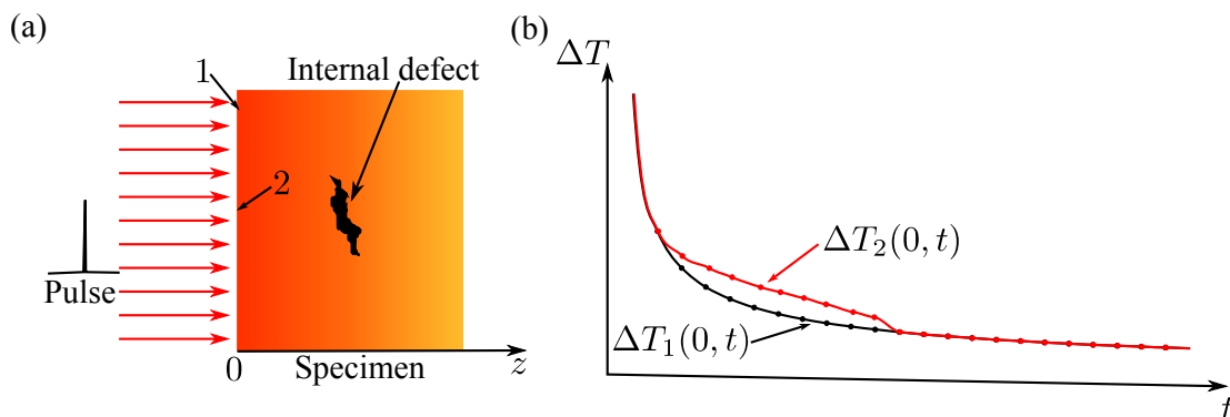
Figure 1.12: (a) Solid specimen containing a buried defect illuminated at its surface z = 0 with a Dirac-like pulse and (b) temperature evolution of the heated surface from a point \Delta T_1(0, t) far from the internal defect and from a point \Delta T_2(0, t) contained in the region of the buried defect.
