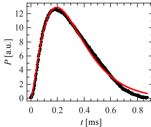
Figure 2.4: Intensity distribution of our Nd-Glass laser pulse. Black dots represent the experimental data and the red curve is the result of fitting to an exponential law.
