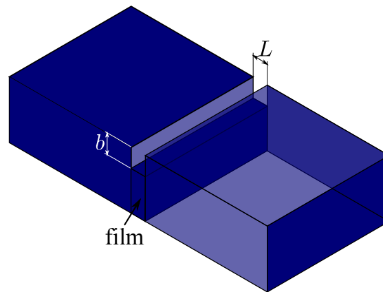
Figure 8.9: Diagram of the semi-infinite vertical crack simulated for the experiment: A thin film of thickness L is sandwiched between two blocks and is buried at a depth b beneath the surface. Blocks and film are made of the same material AISI-304 stainless steel.
